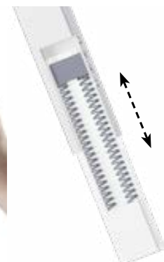
Teleskop-Federsystem
